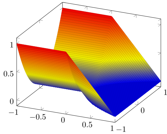
Figure 1: The halfpipe example: f(x) = \max(0, x_2^2 - \max(0, x_1))
